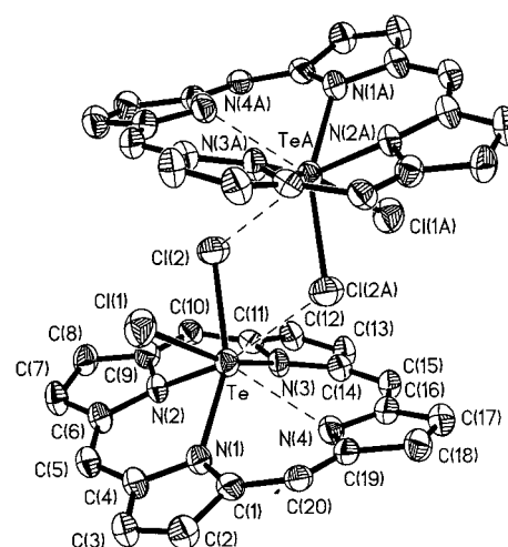
Figure 1. ORTEP plot of [Te(tpp)Cl 2 ]. The meso -tolyl groups and hydrogen atoms are omitted for clarity. Thermal ellipsoids are at the 30% probability level. Selected bond lengths [Å] and angles [°]: Te–N(1) 2.274(3), Te–N(2) 2.094(3), Te–N(3) 2.361(3), Te–N(4) 2.598(3), Te–Cl(1) 2.5108(10), Te–Cl(2) 2.5530(10), Te–Cl(2A) 3.2206(10); N(2)–Te–N(1) 80.53(11), N(2)–Te–N(3) 78.27(10), N(1)–Te–N(3) 118.38(10), N(2)–Te–Cl(1) 89.47(8), N(1)–Te–Cl(1) 78.45(8), N(3)–Te–Cl(1) 156.51(8), N(2)–Te–Cl(2) 89.73(8), N(1)–Te–Cl(2) 157.35(8), N(3)–Te–Cl(2) 78.93(8), Cl(1)–Te–Cl(2) 81.08(4), N(2)–Te–N(4) 122.1(4).
